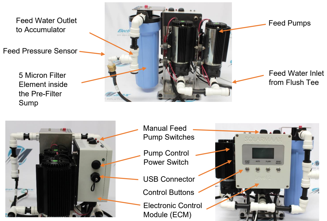
Figure 6: Feed Pump and Assembly
