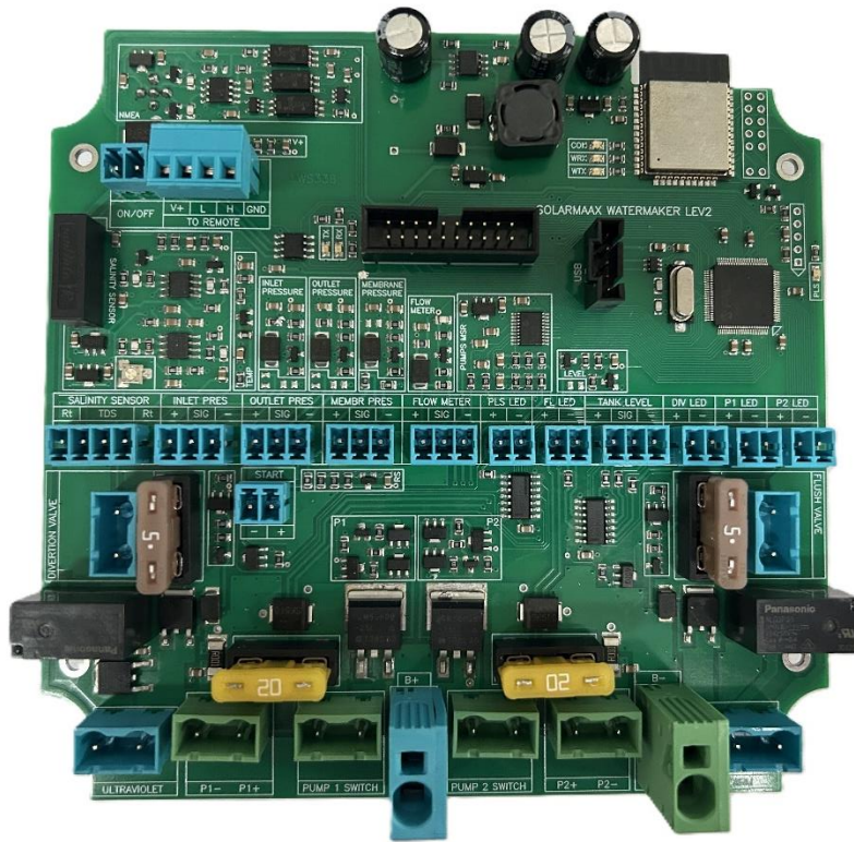
Figure ? Level 2 Circuit Board
