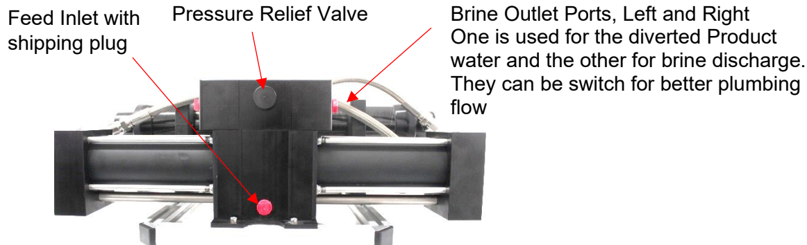
Figure 10: Front View
