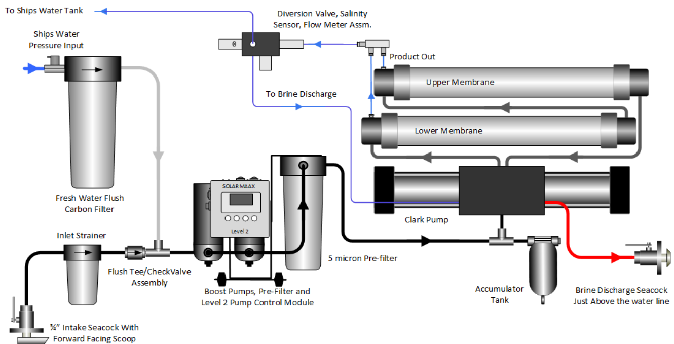
Figure 1: Simplified Component and Plumbing Layout
