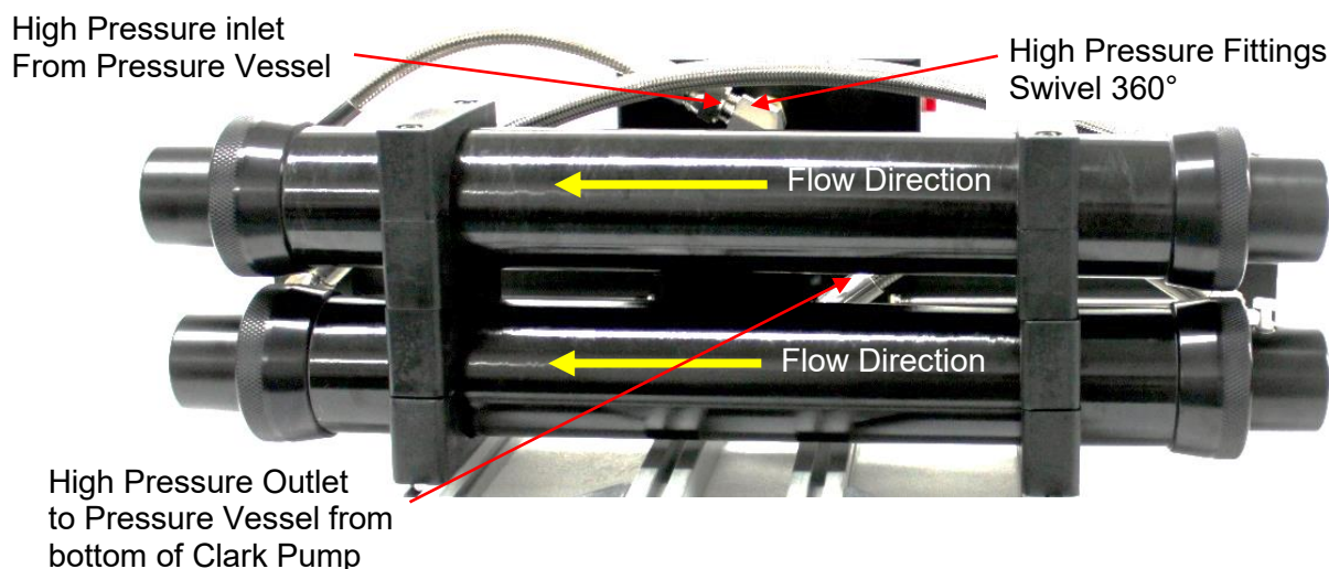
Figure 11: Rear View
