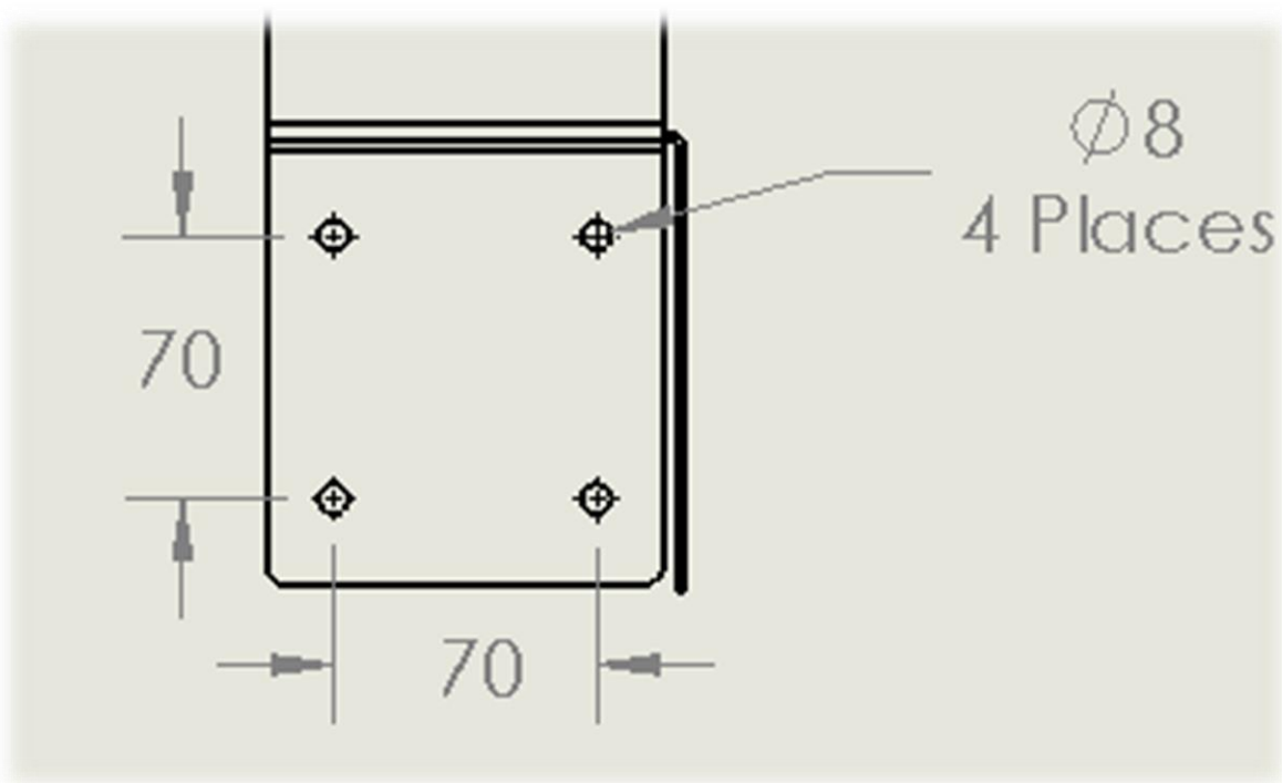
Figure 7: Feed Pump Assembly Foot Mount Drawing
