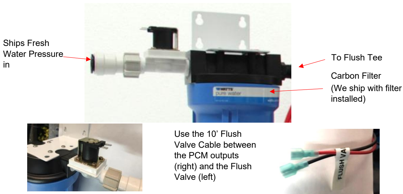
Figure 4: Freshwater Flush Assembly
