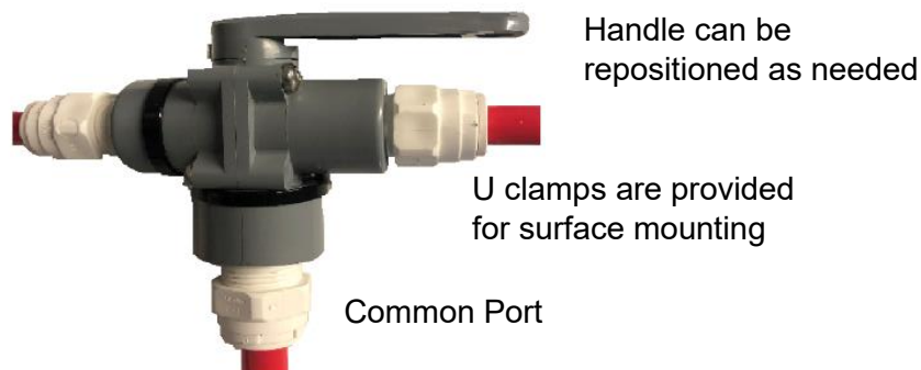
Figure 14: 3-way Service Valves
