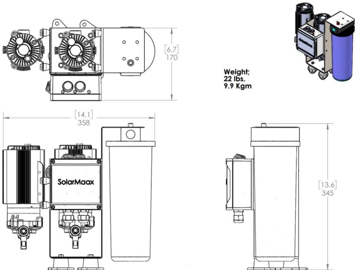
Figure 37: High Pressure Module Dual 21" Membrane Dimensions and Weight
