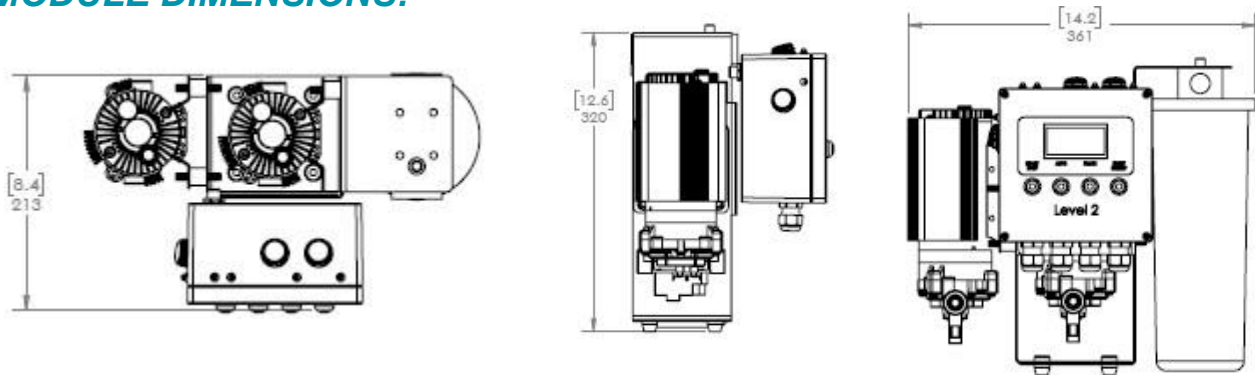
Figure 36: Feed Pump Assembly Dimensions and Weight
