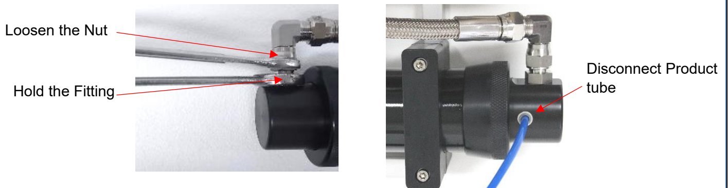
Figure 29: Disconnecting the HP hoses and Product Tube
