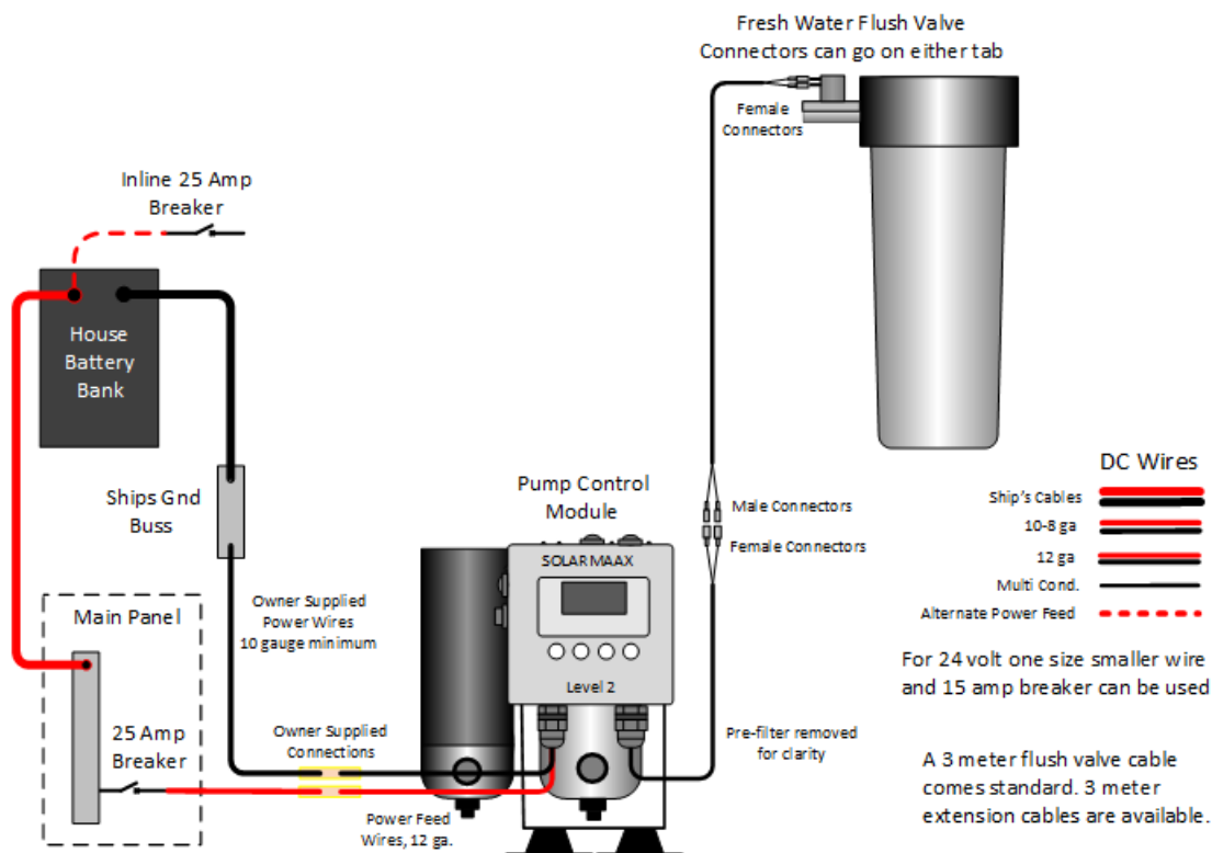
Figure 22: Electrical Diagram
