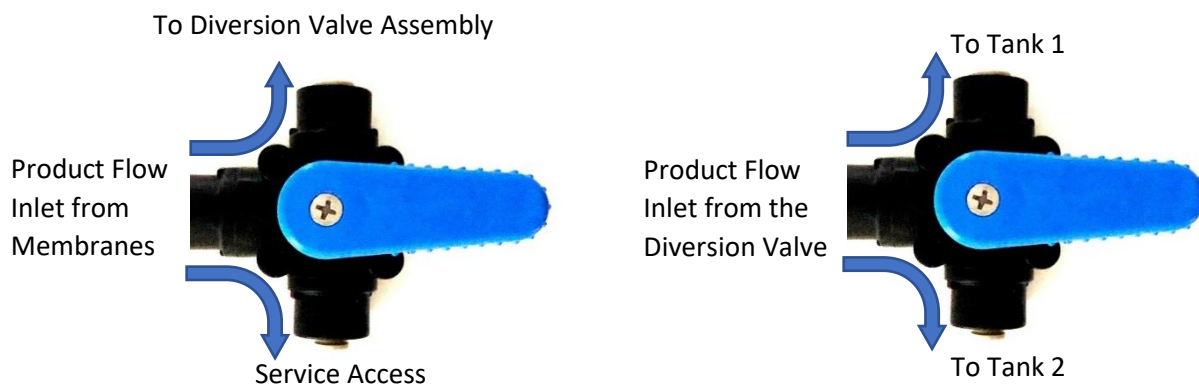
Figure 16: Product 3 Way Valve
