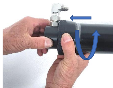
Figure 30: Removing the Pressure Vessel
