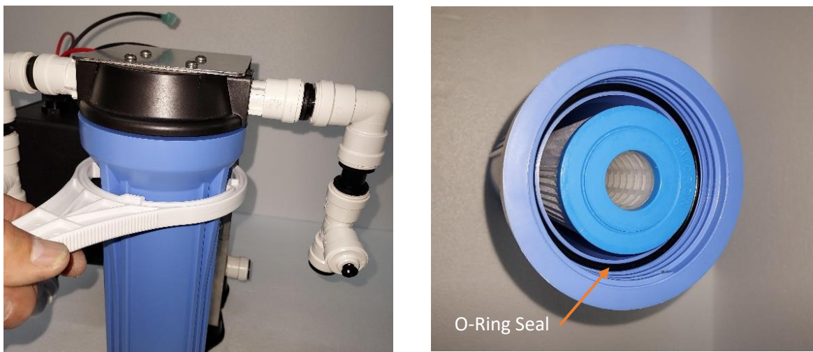
Figure 27: Micron Pre-Filter
