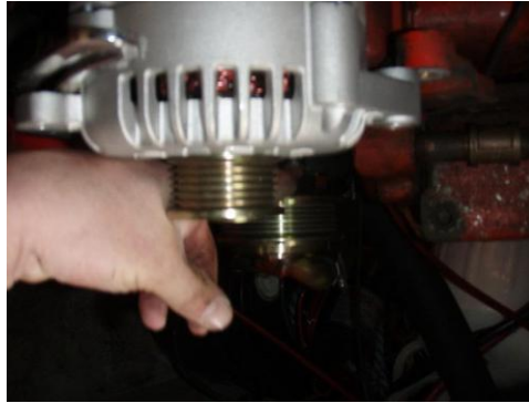
17. Belt Alignment is why the spacer bushing is necessary
